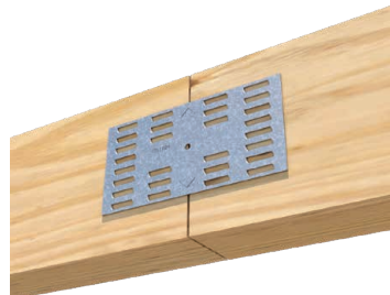
CDTP24 Installation
